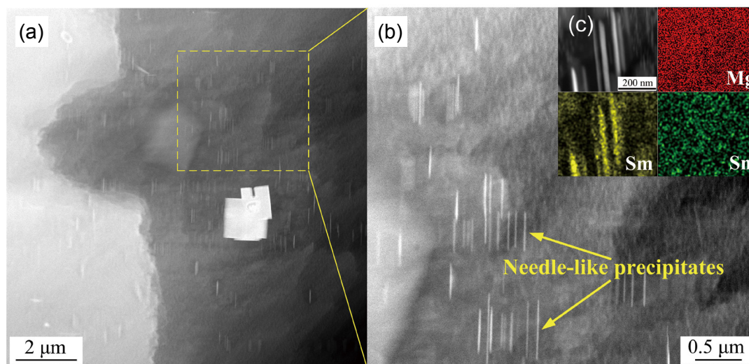
Fig. 7: HAADF-STEM images of peak-aged TE3 alloy: (a) needle-like precipitates within \alpha -Mg matrix; (b) magnified image of precipitates in (a); (c) EDS maps showing the chemical compositions of needle-like precipitates in (b)
