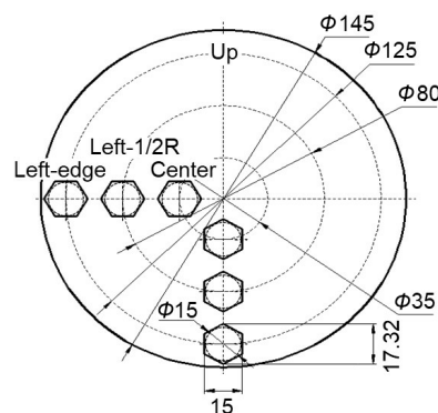
Fig. 1: Samples position for microstructural observation and tensile test
