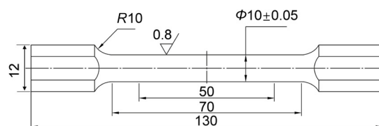
Fig. 2: Schematic diagram of tensile sample (unit: mm)
