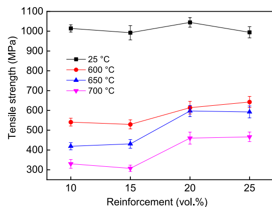
Fig. 6: Tensile strength of (TiC+TiB)/TA15 composites at different temperatures
