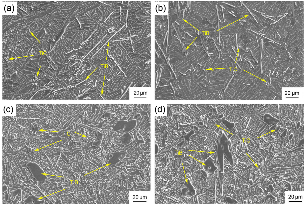
Fig. 4: SEM microstructures of (TiC+TiB)/TA15 composites with various volume fractions of reinforcement: (a) 10vol.%; (b) 15vol.%; (c) 20vol.%; (d) 25vol.%
