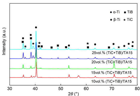
Fig. 3: XRD patterns of (TiC+TiB)/TA15 composites
