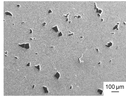
Fig. 1: Microstructure of powder metallurgy ingot
