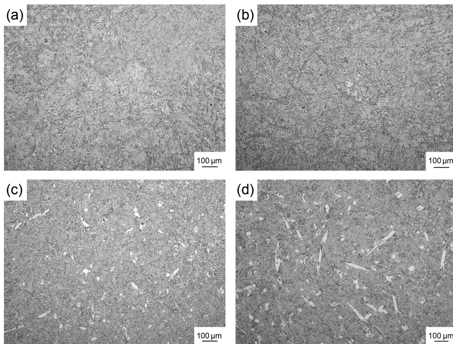
Fig. 2: OM macrostructures showing uniform distribution of reinforcements with various contents: (a) 10vol.%; (b) 15vol.%; (c) 20vol.%; (d) 25vol.%
